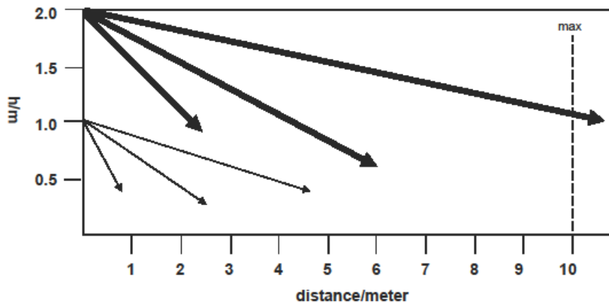
diagram PIR-detection mounted with angle 15°
